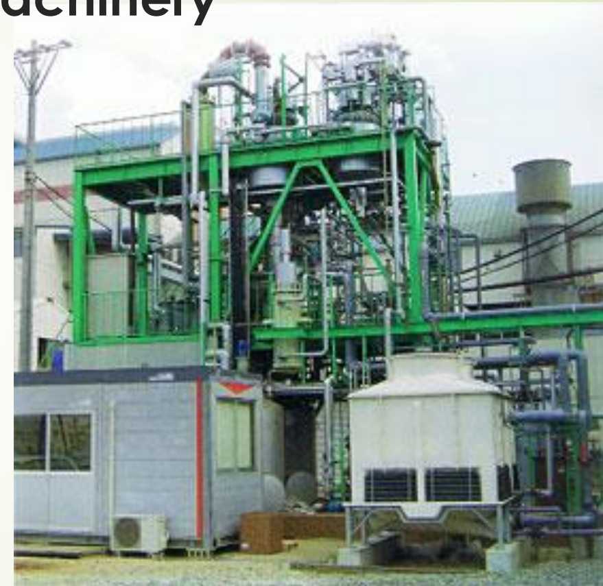
Waste Acid Regenerate Plant
